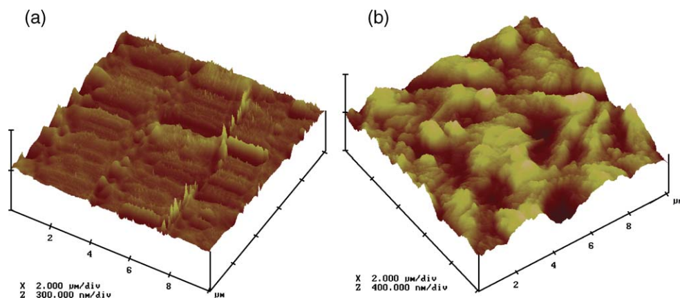
Fig. 3. (a) AFM micrograph of SiO x C y H z thin film deposited on Mg AM60 alloy from 51% TEOS/O 2 discharges at total pressure of 70 Pa and plasma power of 35.9 W and (b) AFM micrograph of bare Mg AM60 alloy.
