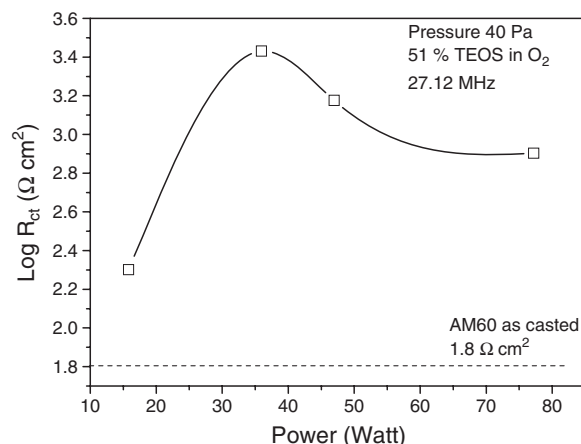
Fig. 5. Charge transfer resistance, R_{ct} , for Mg AM60 alloys coated with SiO_xC_yH_z film as a function of the power dissipated in TEOS/ O_2 discharges. The value of R_{ct} for the uncoated sample is also included.
